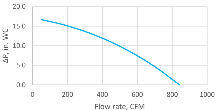
Helios 215 Performance Curve
