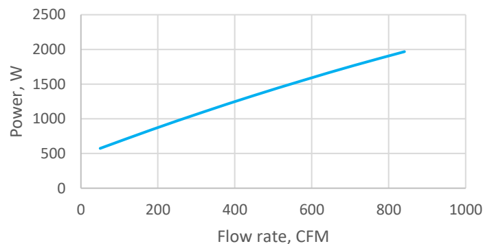
Helios 215 Power Curve
