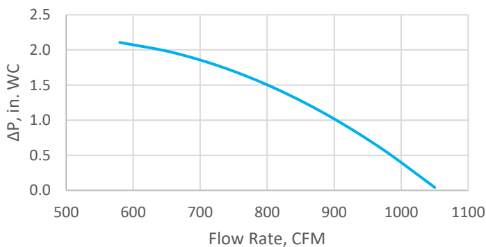
Force 165 Performance Curve
