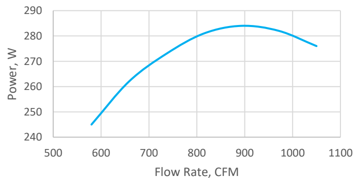
Force 165 Power Curve
