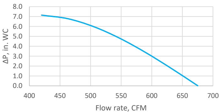
Force 130 Performance Curve
