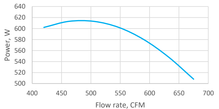
Force 130 Power Curve
