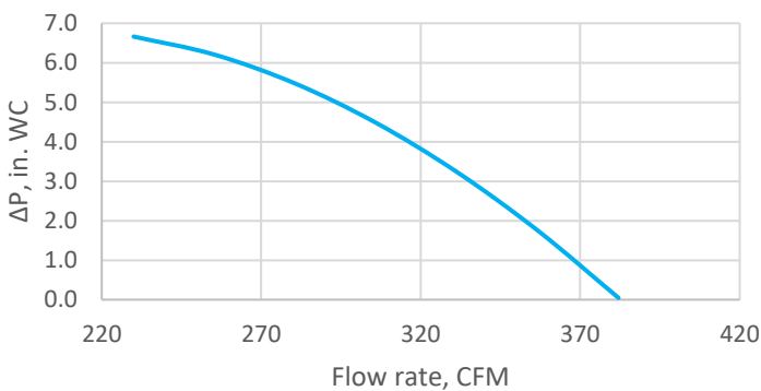
Force 110 Performance Curve
