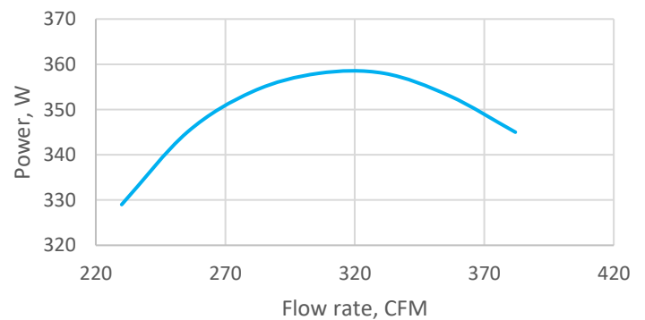
Force 110 Power Curve
